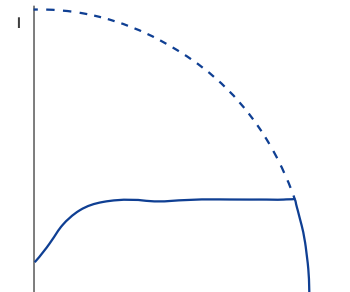
Current diagram with soft starter
